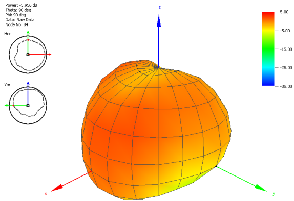
LTE MIMO 1 Radiation Pattern at 2500 MHz
