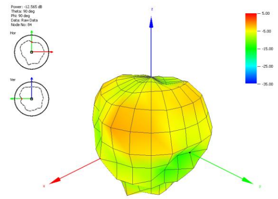
LTE MIMO 2 Radiation Pattern at 3500 MHz
