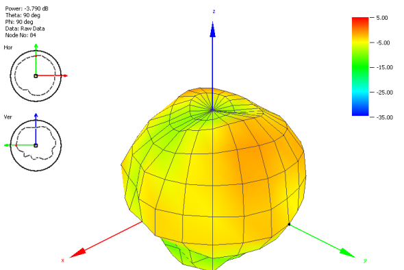
LTE MIMO 2 Radiation Pattern at 2620 MHz
