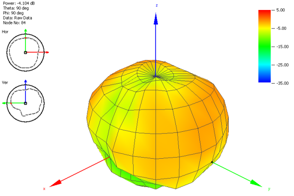
LTE MIMO 2 Radiation Pattern at 2500 MHz
